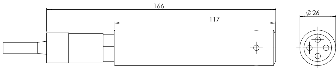
Dimensions ( mm )
